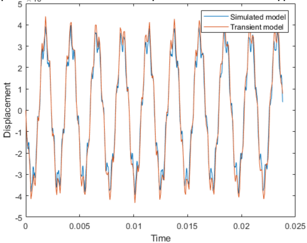
Comparison of full-model simulated response with transient model approximation
